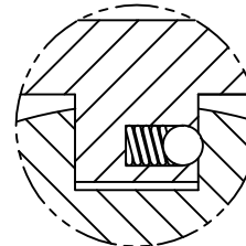
ANTI STATIC DEVICE DETAIL
